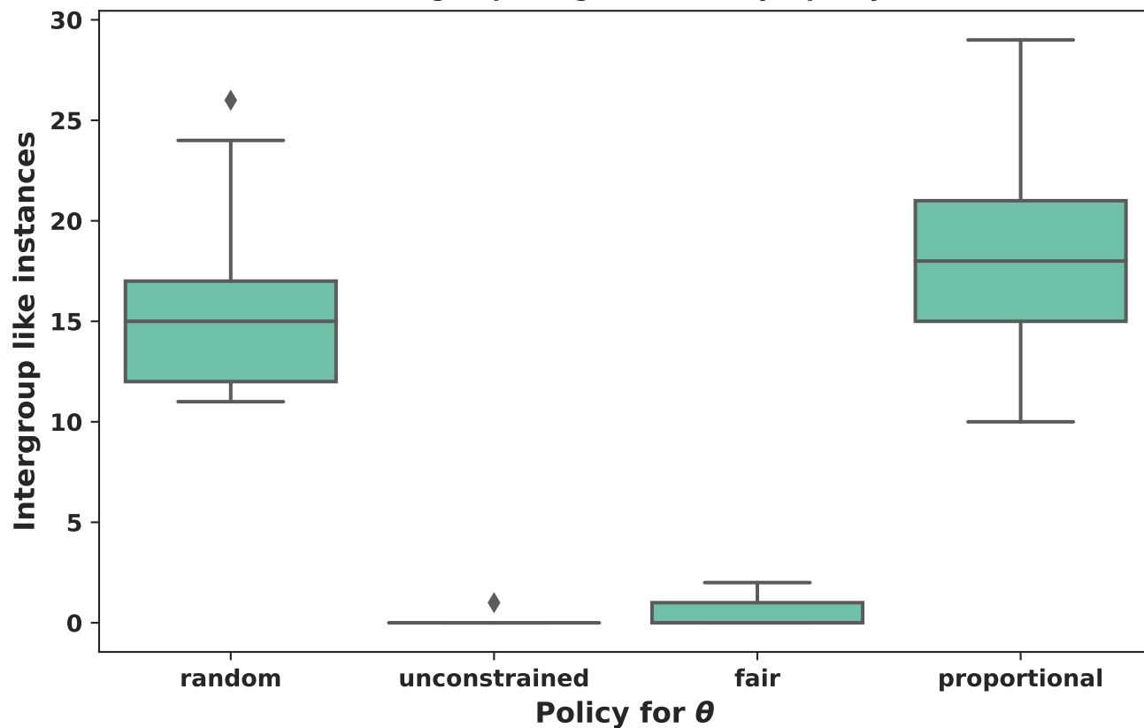
Intergroup liking of articles by \theta policy
